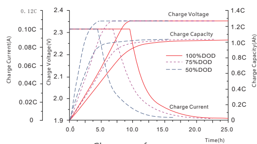
Charge performance
