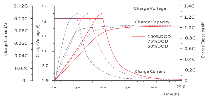
Charge performance
