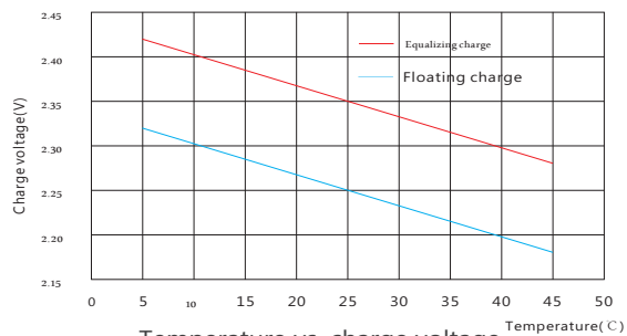
Temperature vs. charge voltage
