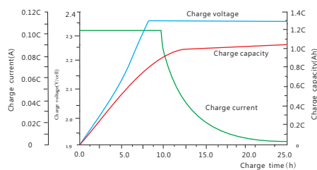
Charge Performance
