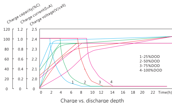
Charge vs. discharge depth
