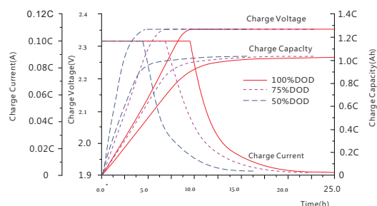
Charge performance
