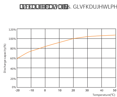
Capacity vs. temperature
