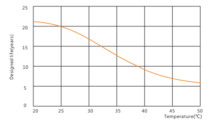
Design life vs. temperature
